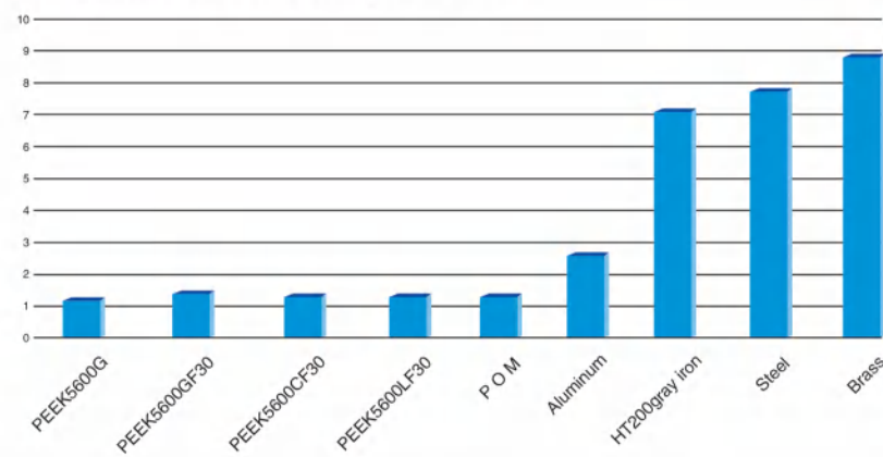
Density values of conventional gear materials:
